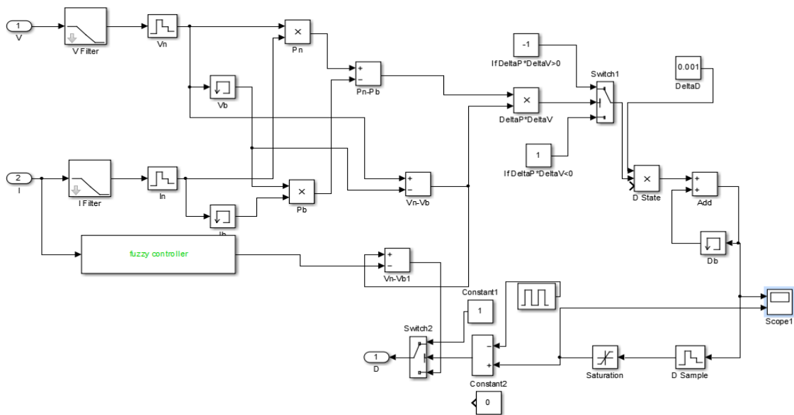
Fig.7. simulation model of Proposed FLC controller for Boost Converter
