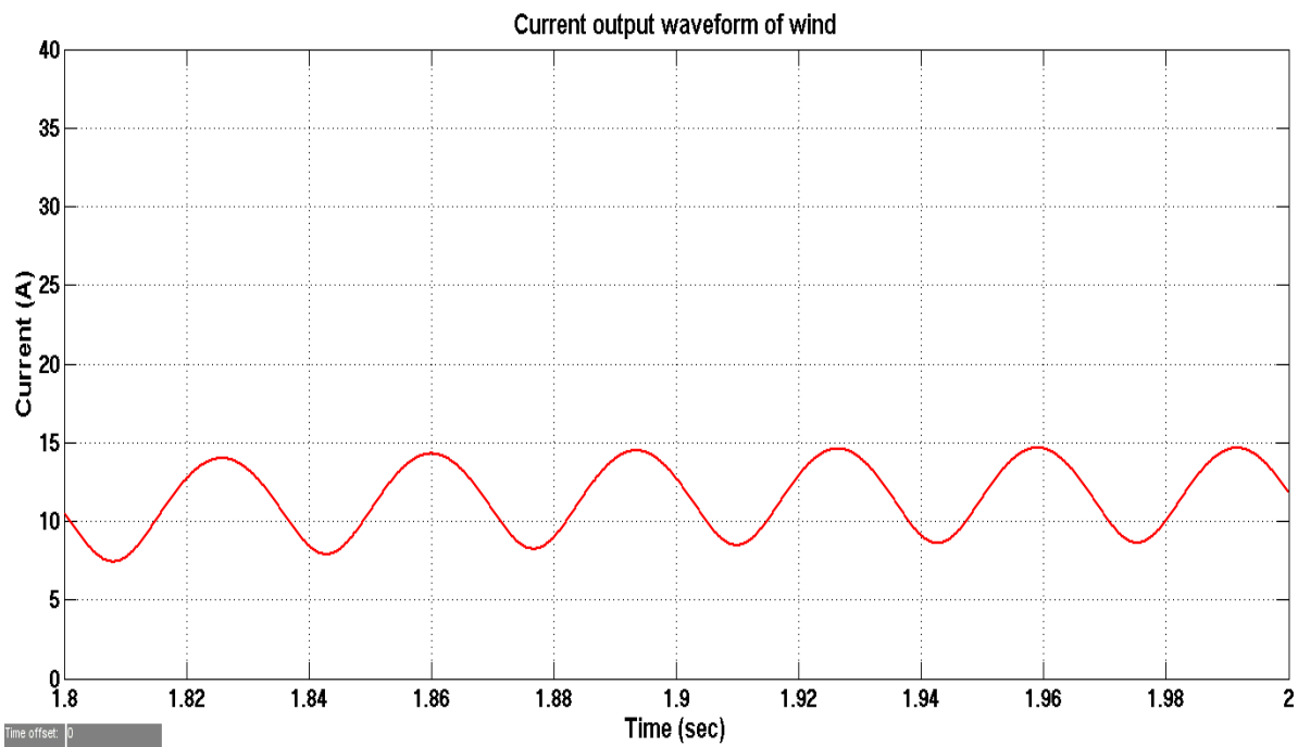
Fig.17.Wind output current waveform
