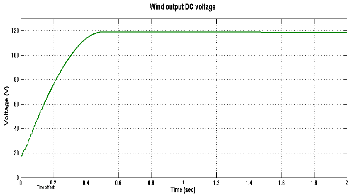
Fig.16.wind power output voltage waveform
