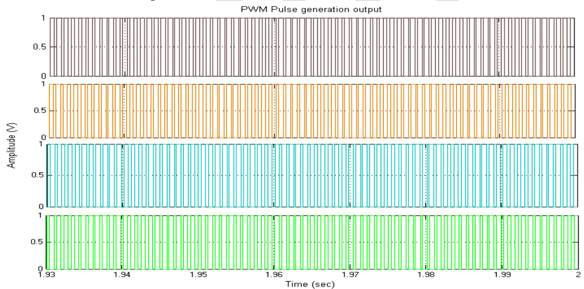
Fig.14. PWM signal waveform for Inverter control
