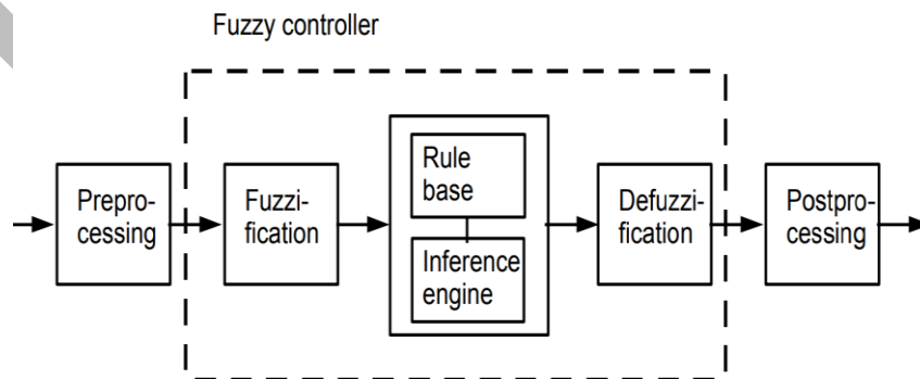
Fig.2. Fuzzy controller Working Method
