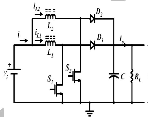
Fig.3. Interleaved boost converter
