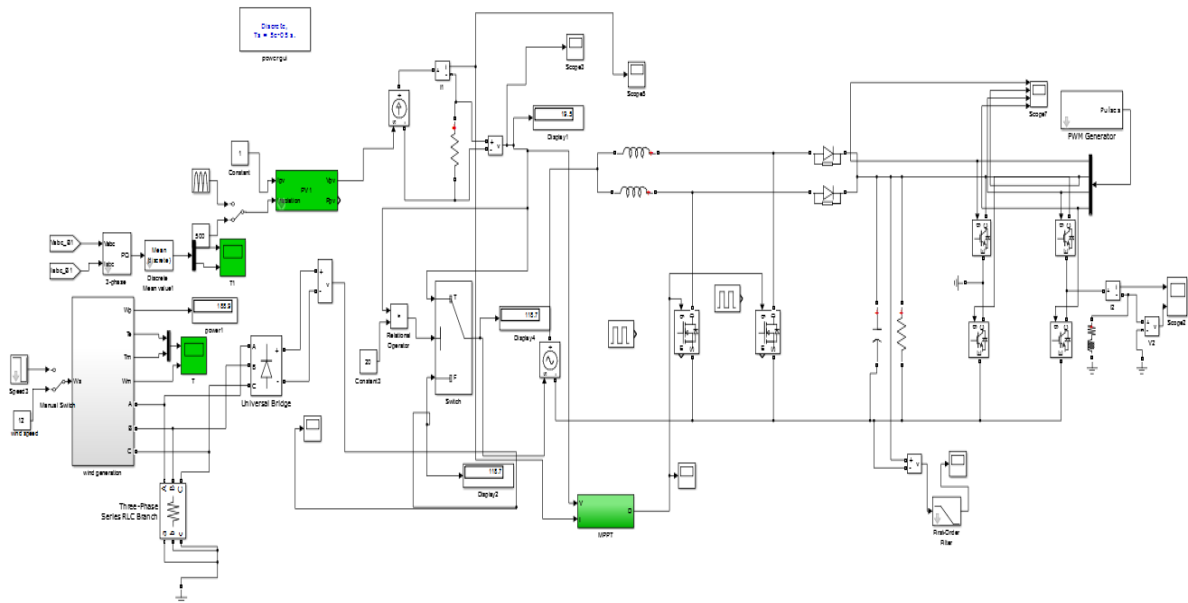
Fig.4. Simulation model for proposed hybrid wind solar generation system
