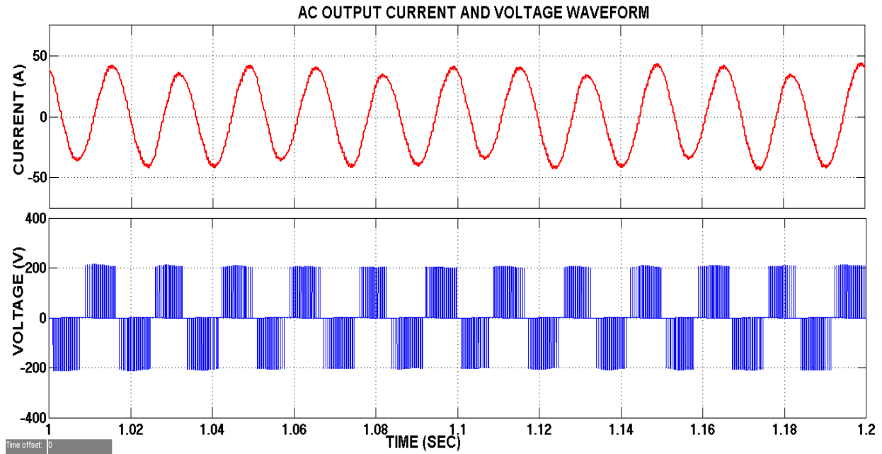
Fig.24.Voltage and current output waveform for PV with Battery
