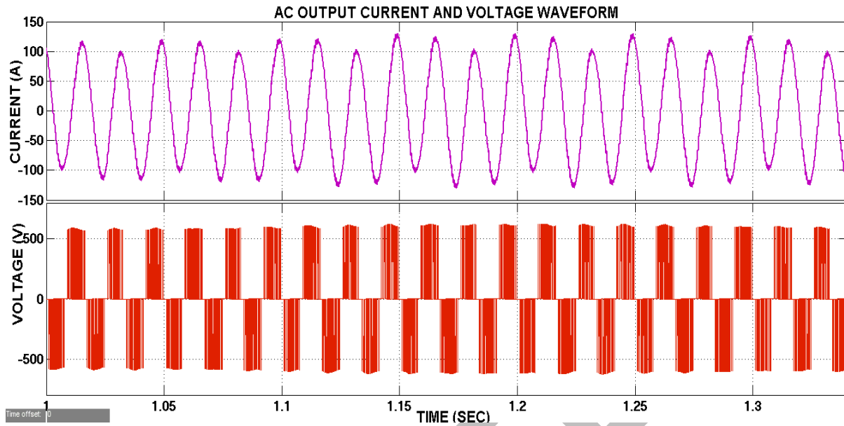
Fig.15. AC output Voltage Waveform
