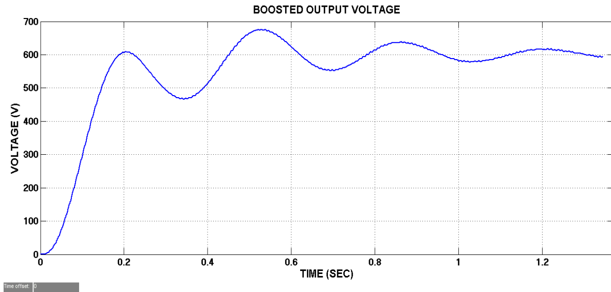
Fig.13. Boost converter output Voltage waveform
