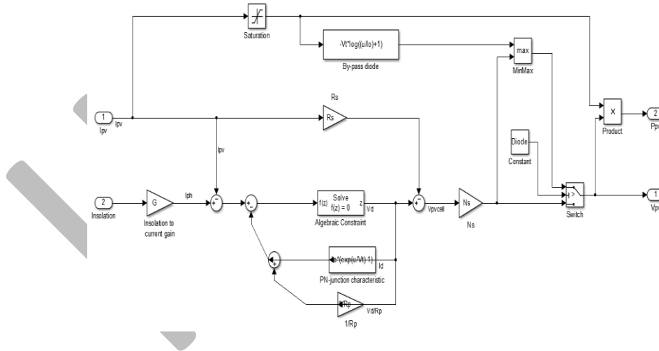
Fig.5. Simulation model of solar power generation
