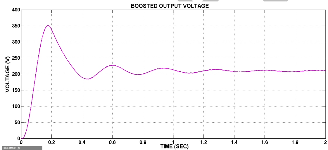
Fig.23.Boosted output voltage waveform
