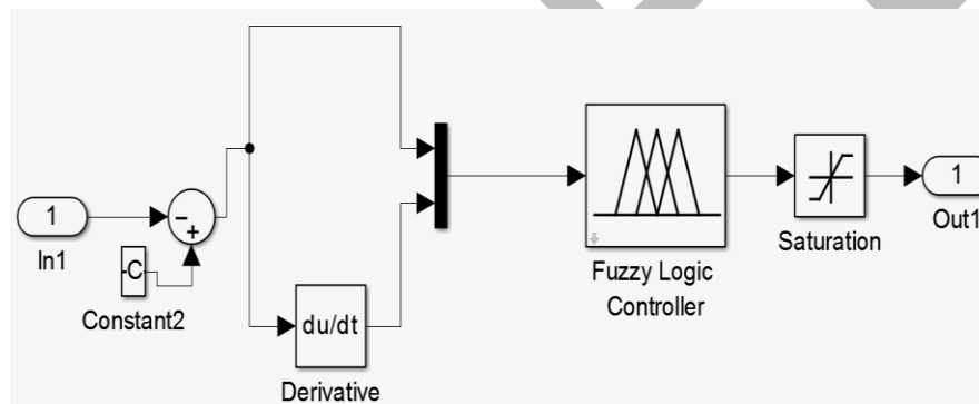
Fig.9. Simulation model of Implemented Fuzzy Logic Controller
