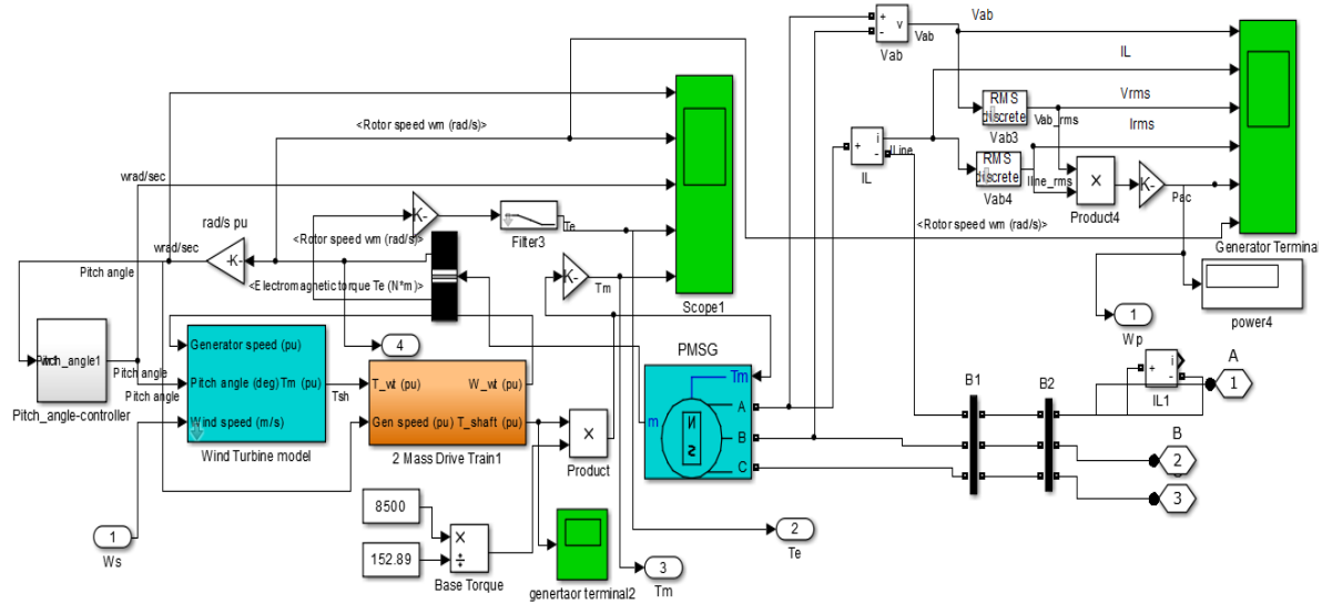
Fig.6. PMSG base wind turbine simulation model
